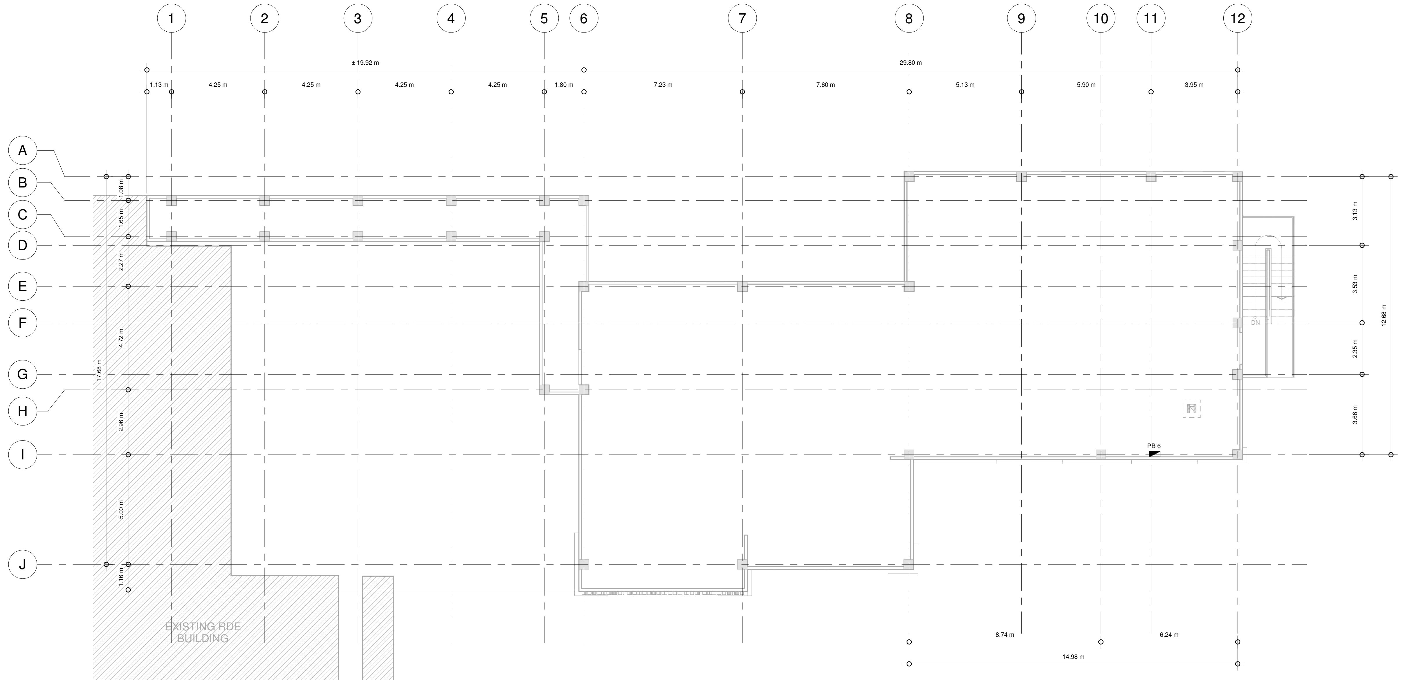
1 ROOF DECK PANEL BOARD PLAN 1 : 100 meters
